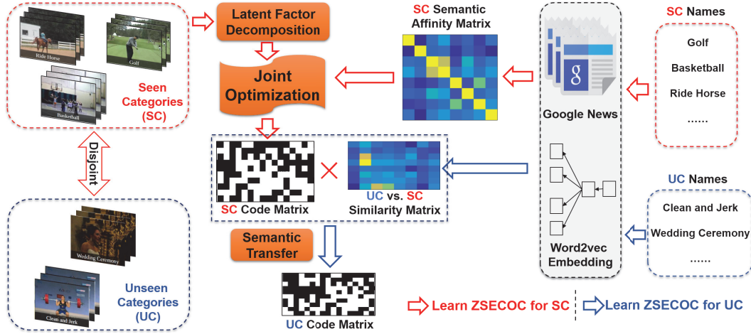
Figure 2. The flow chart of ZSECOC. We design discriminative ZSECOC for seen categories that is both semantics-preserving and data-driven. A joint optimization framework is proposed to solve the resultant challenging problem. We learn the ZSECOC for unseen categories through a simple yet effective semantic transfer strategy. Black and white entries of the code matrix indicate ‘1’ and ‘-1’, respectively.
