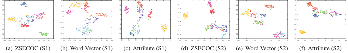
Figure 6. t-SNE [36] visualization between different embeddings of unseen categories w.r.t. two representative (S)plits on Olympic Sports.
